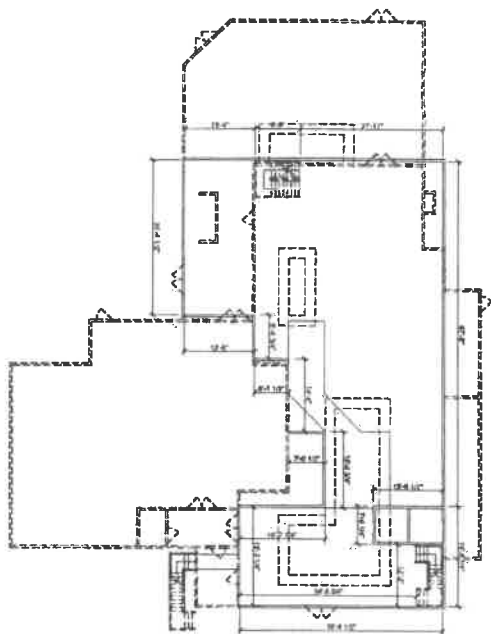
2 EXISTING SECOND FLOOR PLAN Scale: \frac{3}{8}" = 1'-0"
