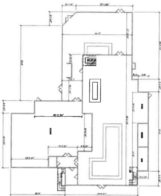
1 EXISTING FIRST FLOOR PLAN Scale: \frac{3}{8}" = 1'-0"
